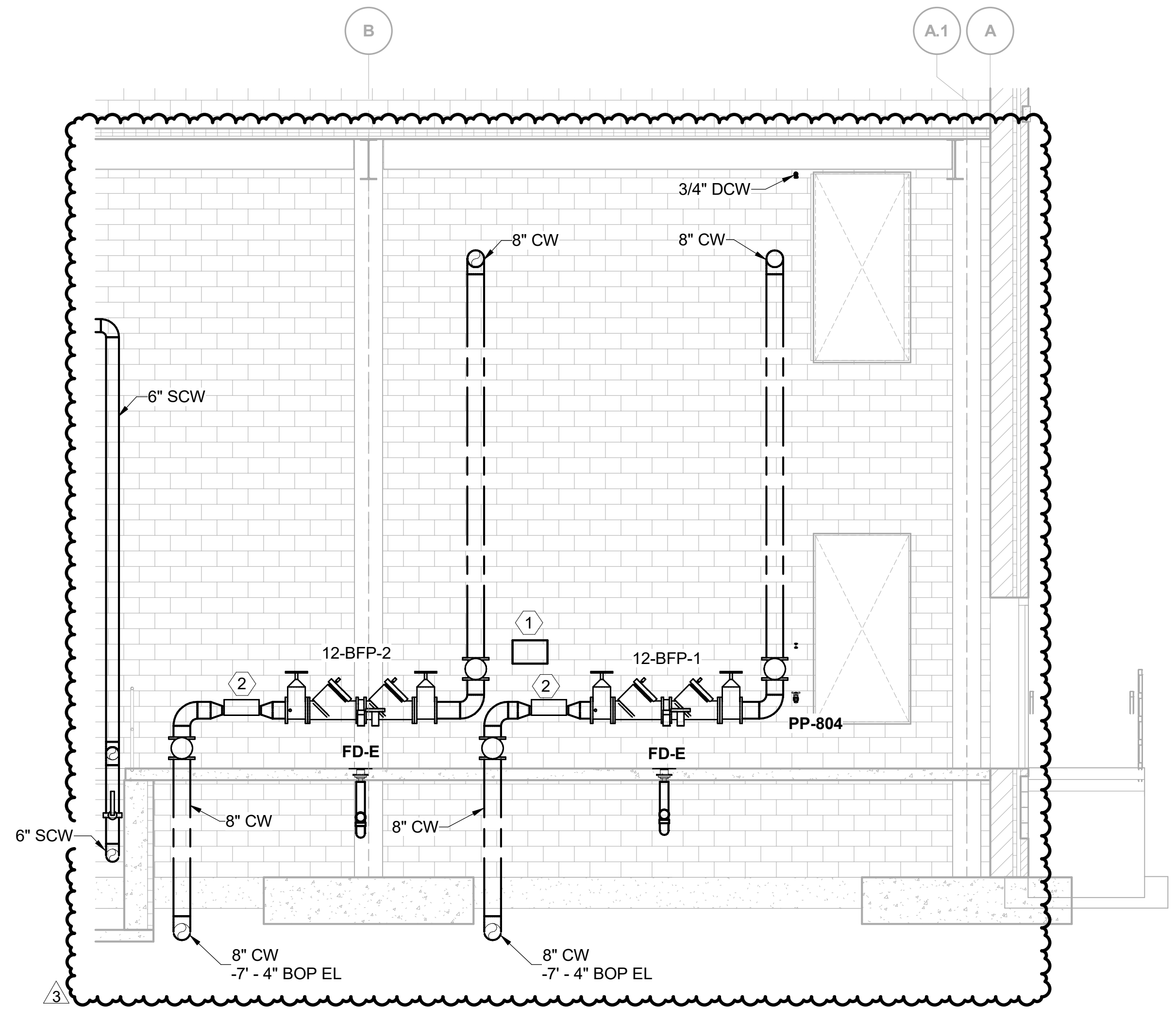
SECTION 1 BFP SECTION PL101 SCALE IN FEET 0 2' 4' 8'
